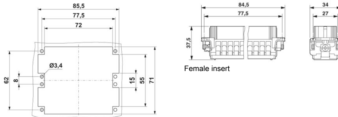
Female insert
